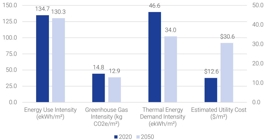
Figure 21 - 2020 and 2050 Targeted Performance
