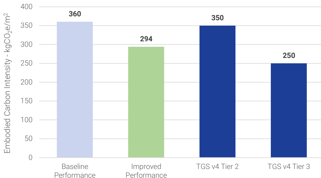
Figure 20 - Estimated Embodied Carbon Benchmarked Performance
