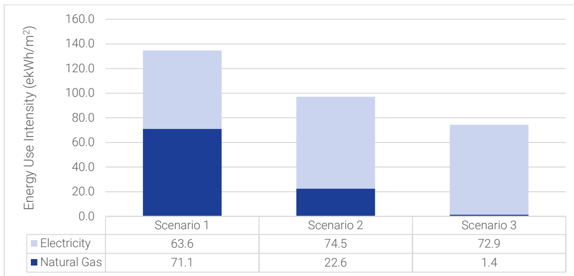
Figure 3 - Predicted Energy Consumption by End-Use
