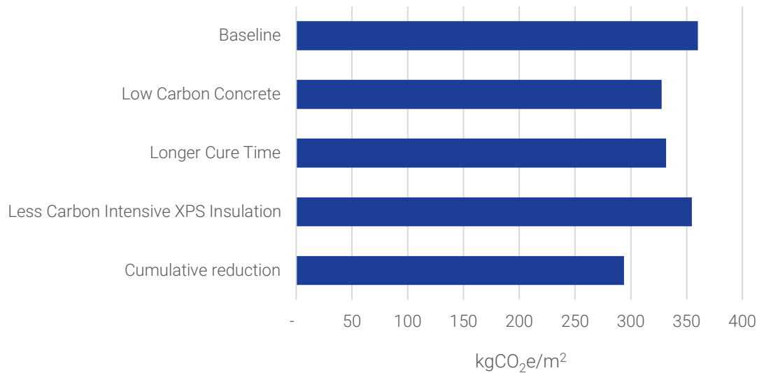
Figure 19– Embodied Carbon Reduction Summary Graph
